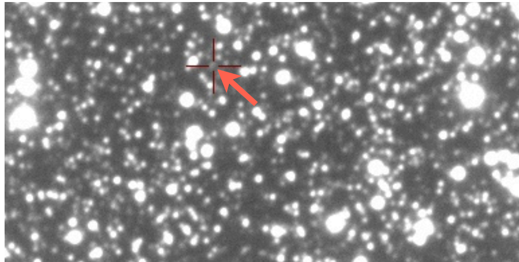
OGLE-III template (composite 2001-2003) progenitor at I=19.7 mag
