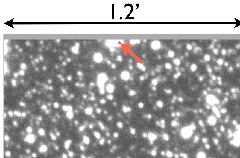
OGLE-IV, 11 Mar 2010, the earliest frame about I=11 mag (edge of the frame)
