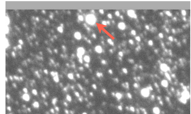
OGLE-IV, 25 April 2010 about I=13.8 mag
