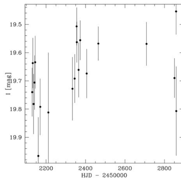
light curve 2001-2003
